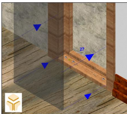
Fig. 4.1 – Glass installation
