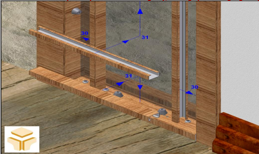
Fig. 4.4.2 – Glass fixation (installing edging strips holding on the glass)
